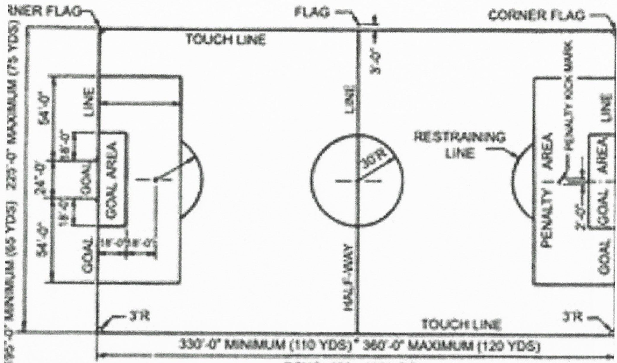
PLAYING FIELD LAYOUT
